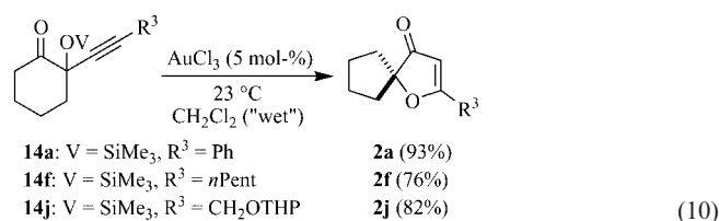
Scheme 3. Stereospecific course of the cyclization-migration reactions.
